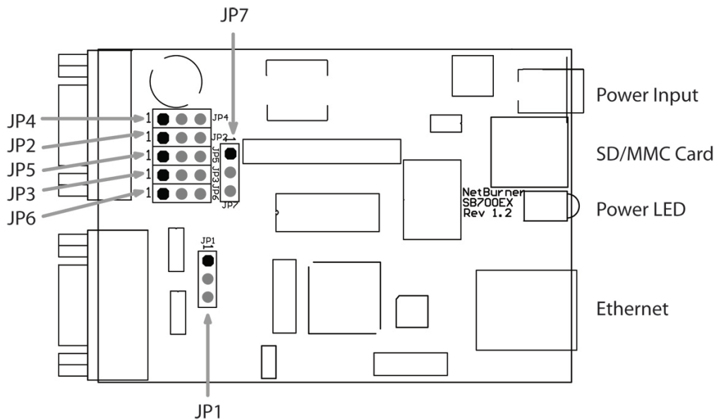
Figure 2: SB700EX
