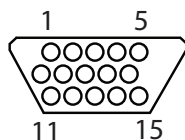
Figure 1: Pin locations for Multi-function I/O Connector (Port 1)
